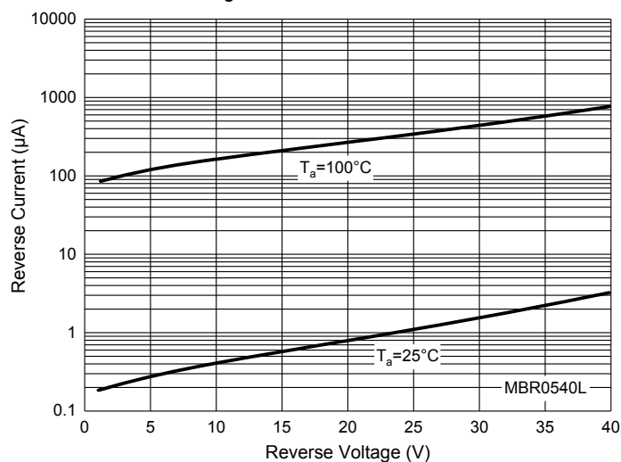
Fig. 6 - Reverse Characteristics
