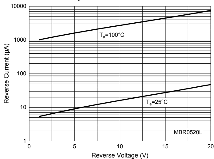
Fig. 4 - Reverse Characteristics
