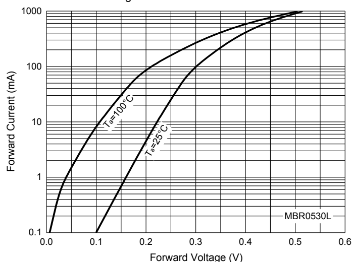
Fig. 2 - Forward Characteristics
