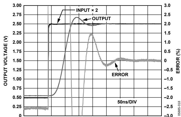
Figure 20. Settling Time
