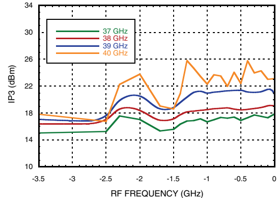
Input IP3, USB vs. Control Voltage
