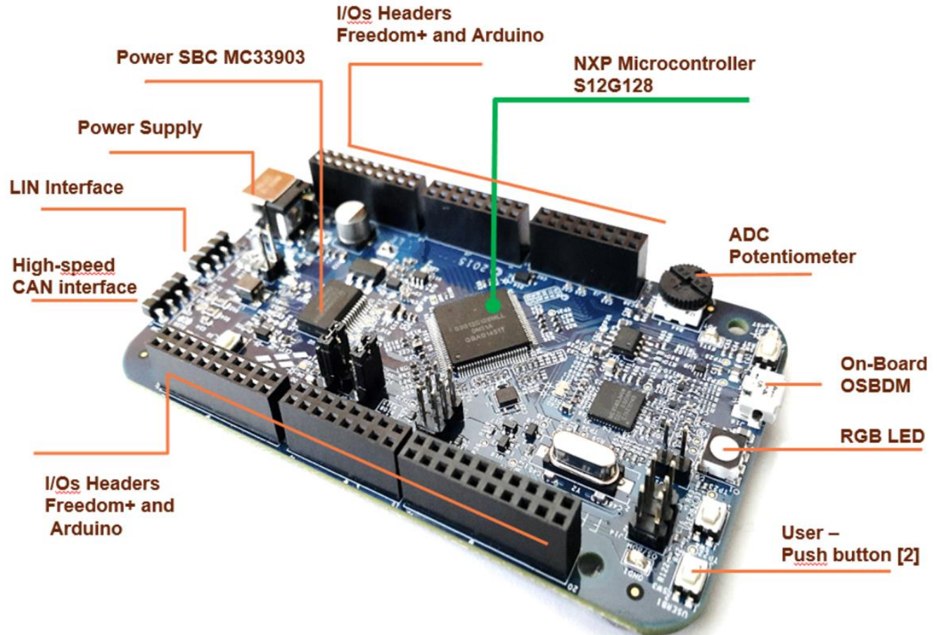
DEVKIT-S12G128 Features
