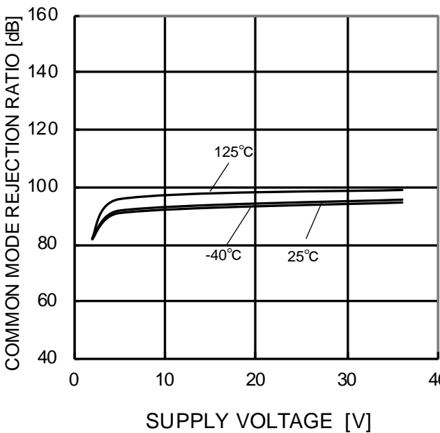
Figure 40. Common Mode Rejection Ratio – Supply Voltage
