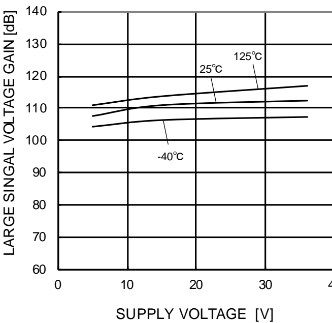
Figure 38. Large Signal Voltage Gain – Supply Voltage
