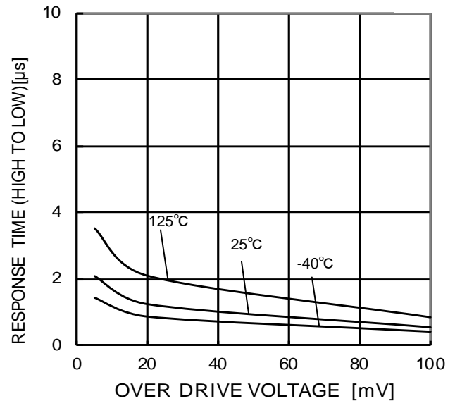
Figure 46. Response Time (High to Low) – Over Drive Voltage (VCC=5V, VRL=5V, RL=5.1kΩ)
