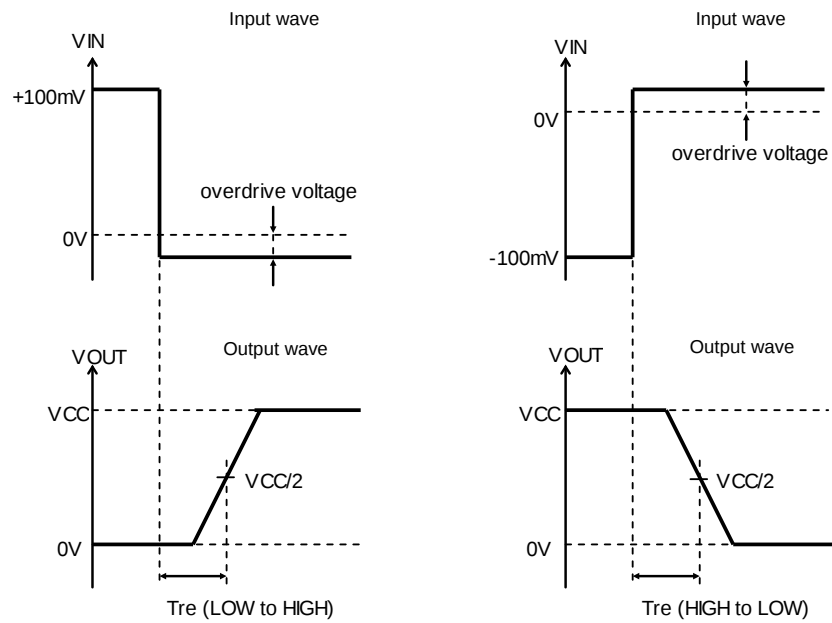
Figure 52. Response Time
