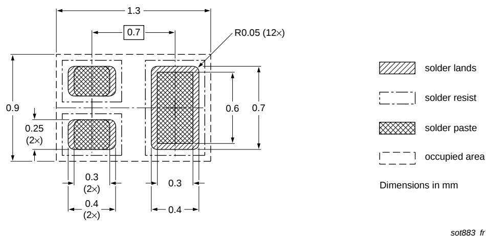
Fig 17. Reflow soldering footprint PDTA144EM (SOT883/SC-101)
