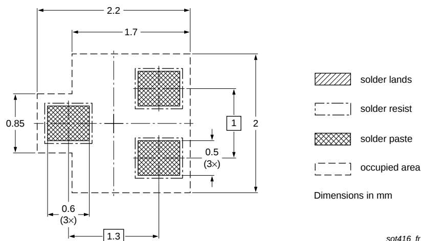
Fig 16. Reflow soldering footprint PDTA144EE (SOT416/SC-75)
