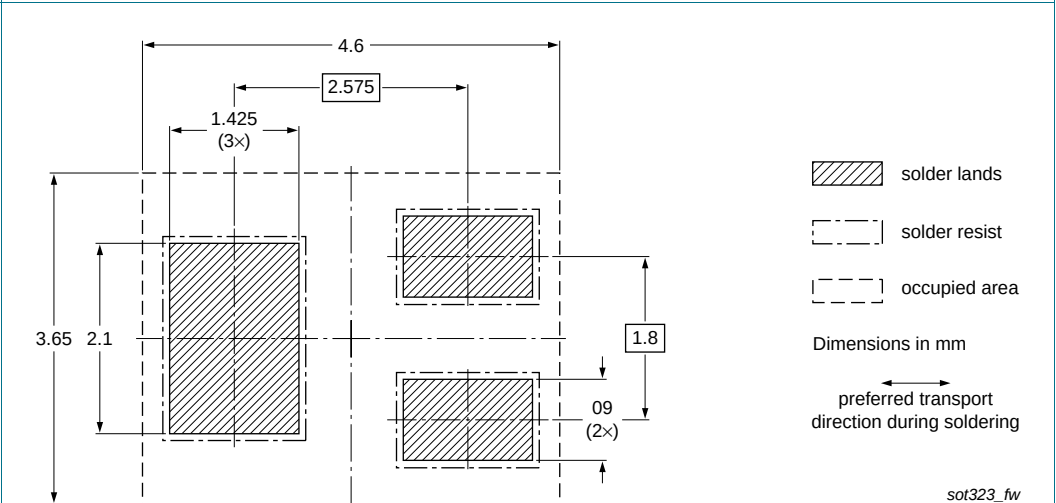
Fig 20. Reflow soldering footprint PDTA144EU (SOT323/SC-70)
