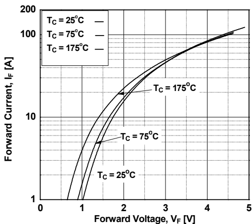
Figure 21. Forward Characteristics
