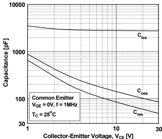
Figure 9. Capacitance Characteristics
