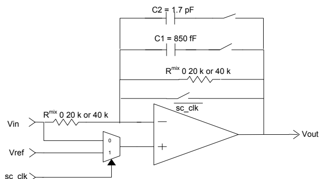
Figure 8-12. Mixer Configuration
