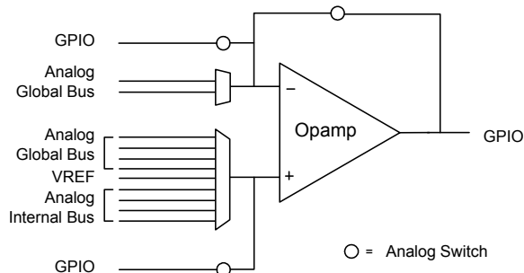
Figure 8-6. Opamp
