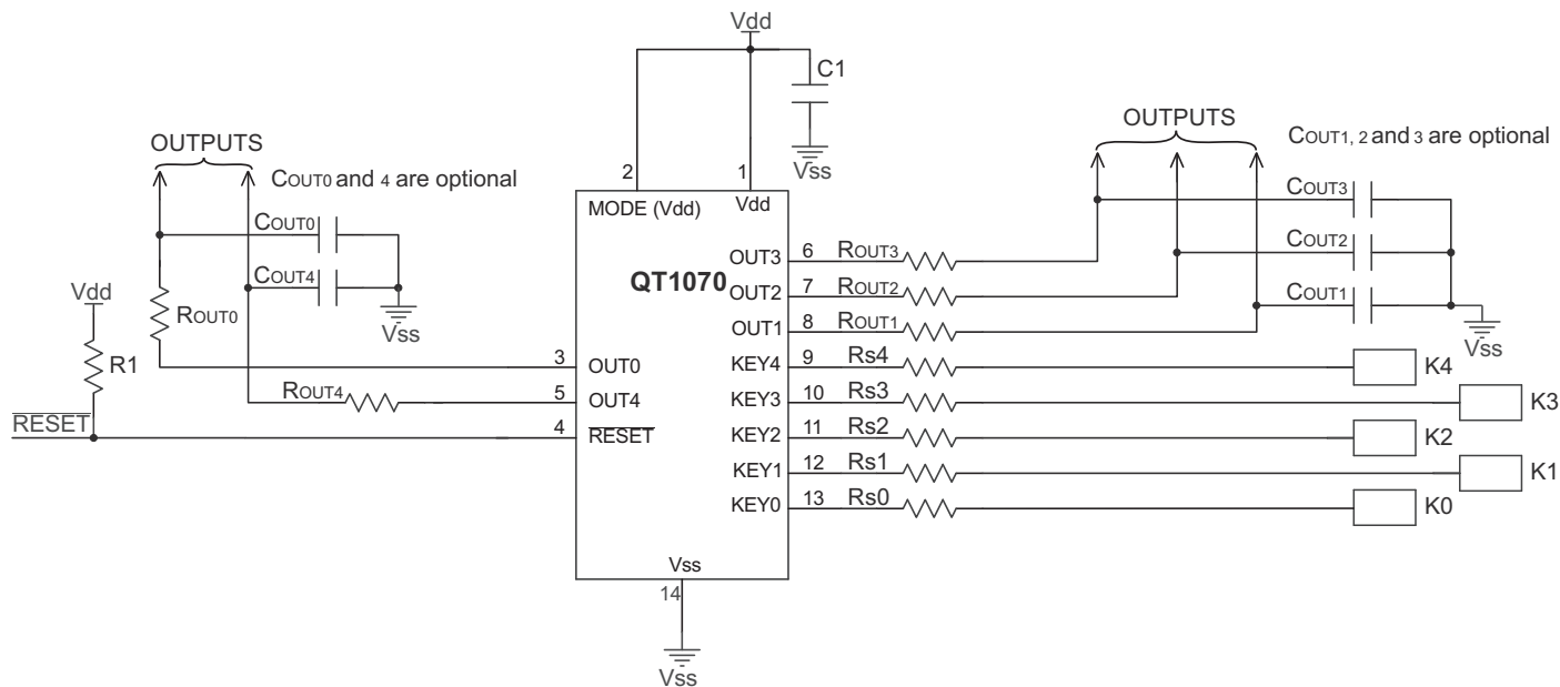
Figure 1-2. Typical Circuit – Standalone (14-pin SOIC)
