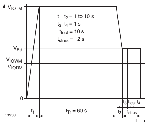
Figure 5. Test pulse diagram for sample test according to DIN EN 60747-5-2(VDE0884)/ DIN EN 60747-5; IEC60747
