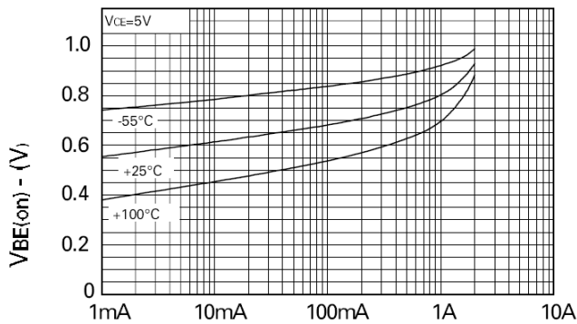
IC-Collector Current
