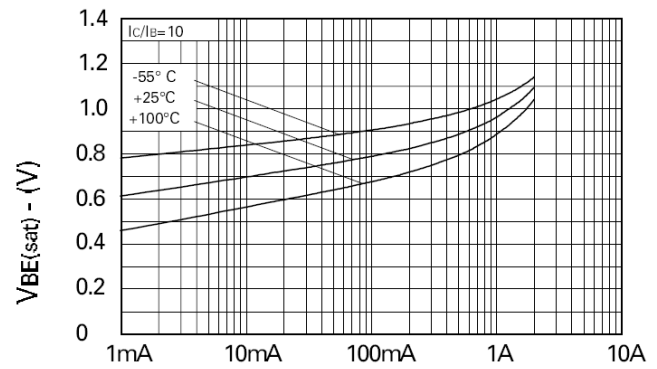
IC-Collector Current
