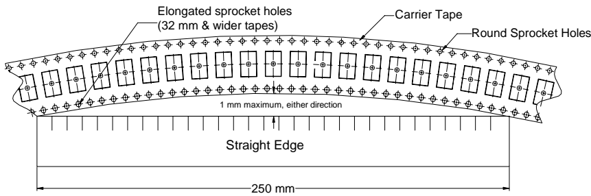
Figure 7 – Maximum Camber
