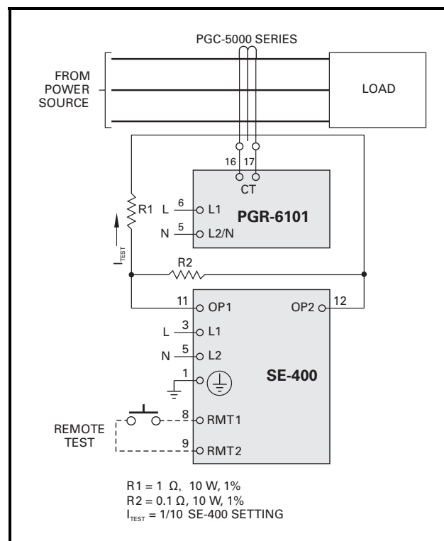
FIGURE 8. Ground-Fault-Test Circuit.
