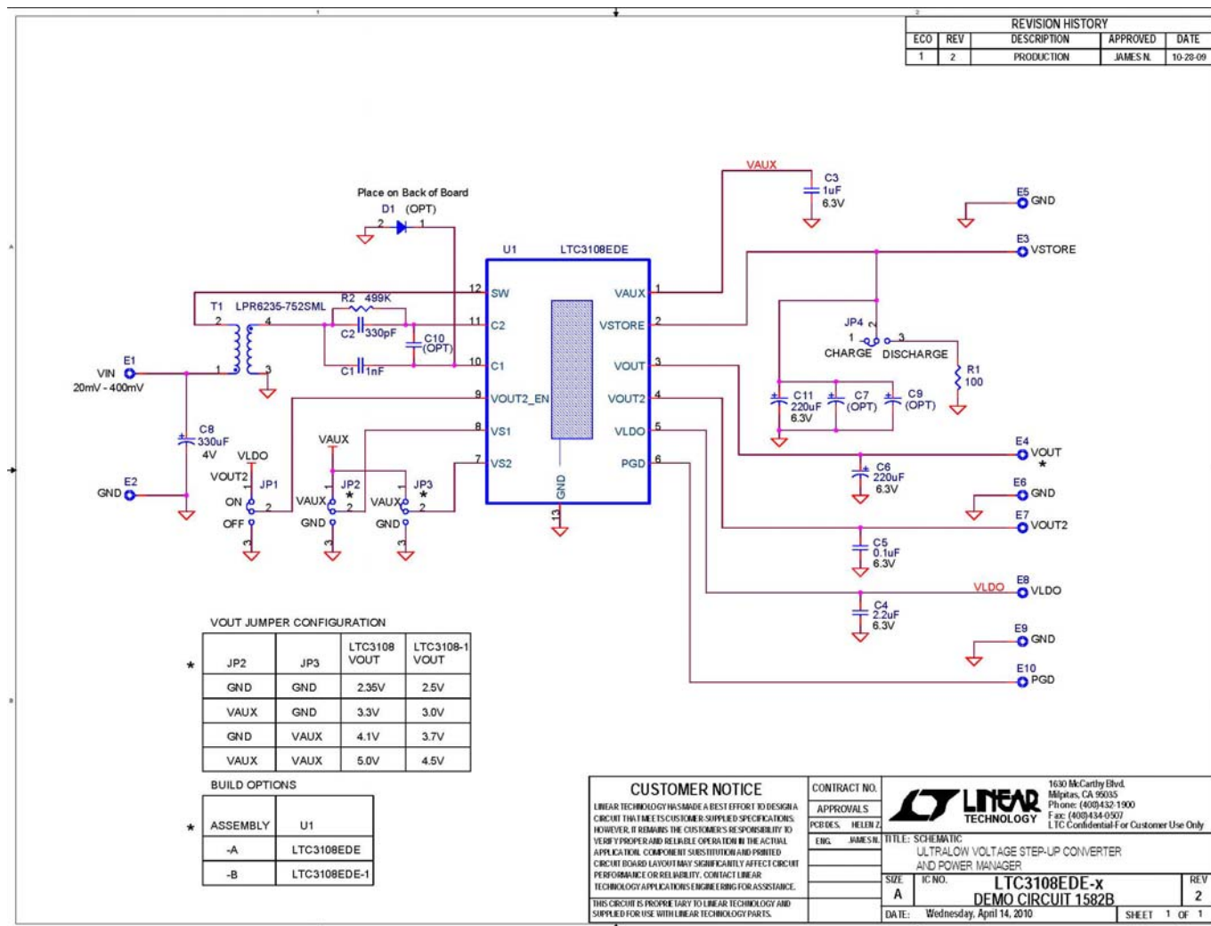
Figure 3. Circuit Schematic
