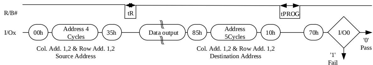
Figure 8.6 Page Copy-Back Program Operation
