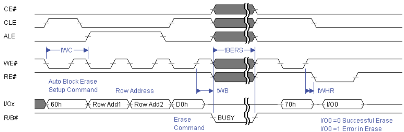
6.14 BLOCK ERASE OPERATION
