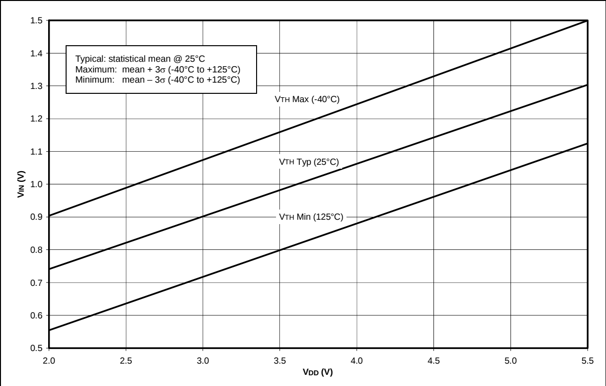
FIGURE 18-20: MINIMUM AND MAXIMUM V_{IH} vs. V_{DD} (TTL INPUT, -40^{\circ}C TO +125^{\circ}C )
