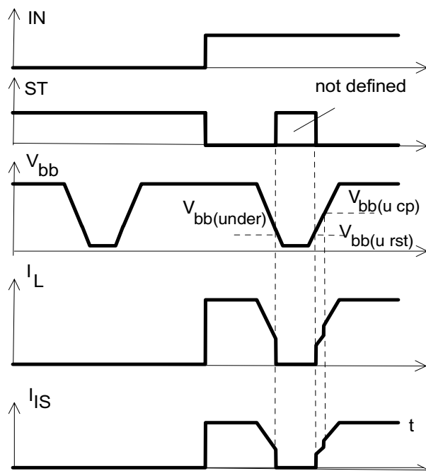
Figure 6a: Undervoltage:
