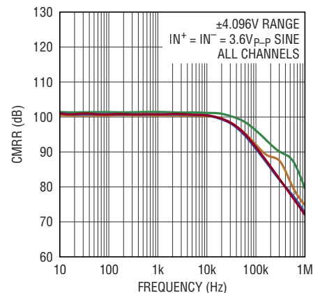
CMRR vs Input Frequency and Channel
