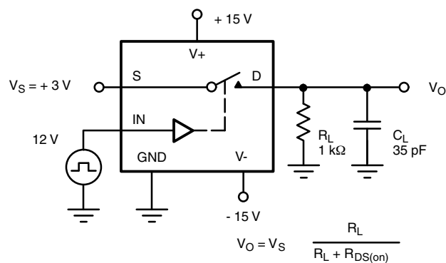
Figure 2. Switching Time
