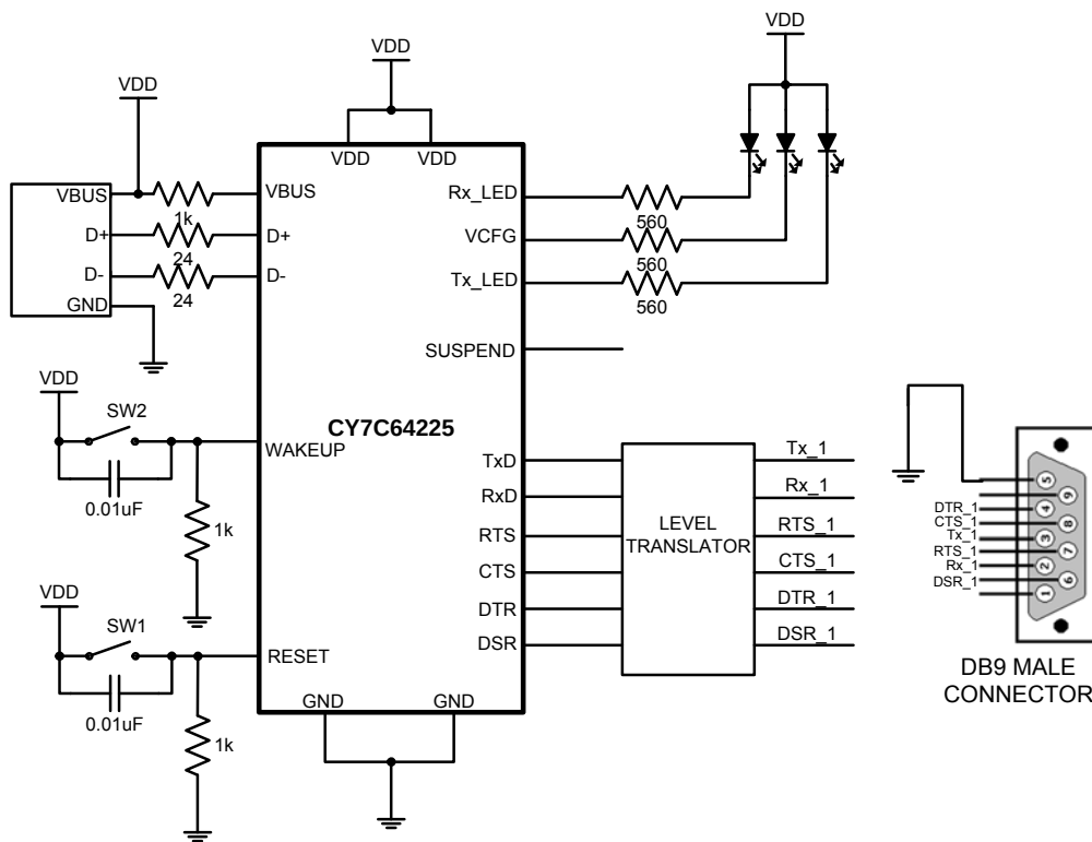
Figure 6. USB to RS-232 Converter Configuration
