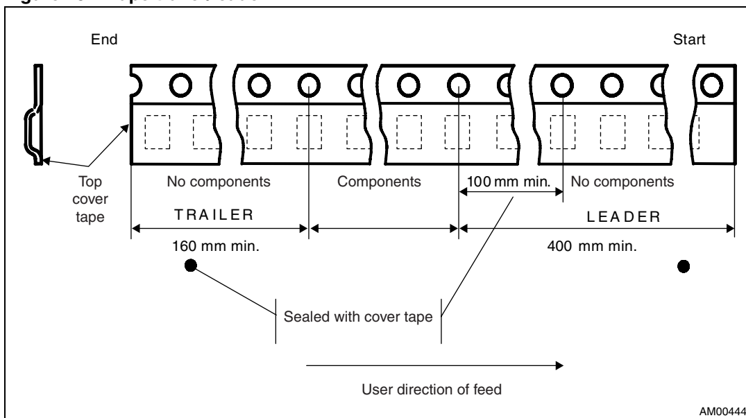
Figure 15. Tape trailer/leader
