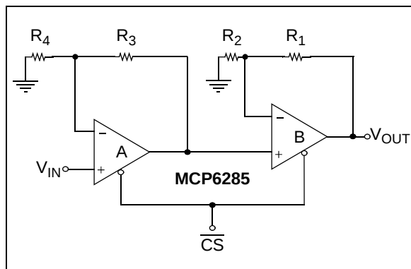
FIGURE 4-11: Cascaded Gain Circuit Configuration.
