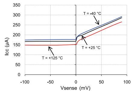
Figure 6: Supply current vs. Vsense
