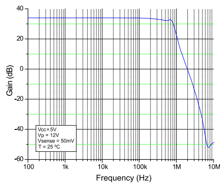
Figure 13: Bode diagram
