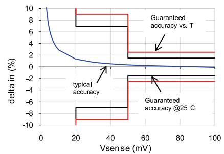
Figure 4: Output voltage accuracy vs. Vsense
