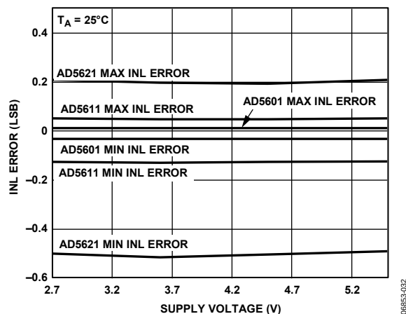
Figure 33. INL vs. Supply Voltage at 25°C
