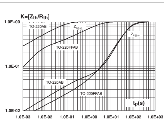
Figure 5. Relative variation of thermal impedance versus pulse duration
