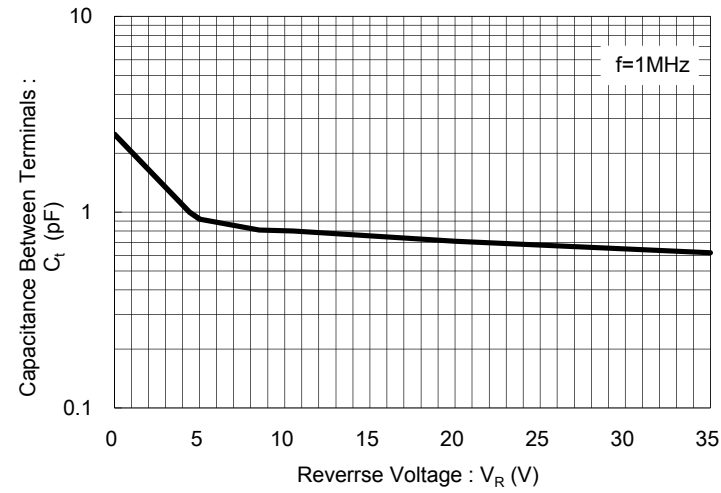
V_R - C_t Characteristics
