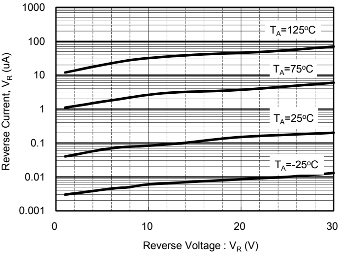
V_R - I_R Characteristics
