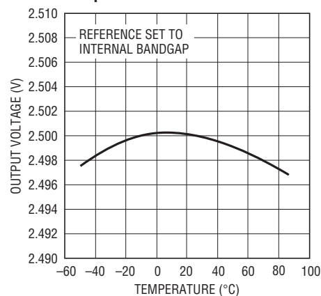
Full-Scale Output Voltage vs Temperature
