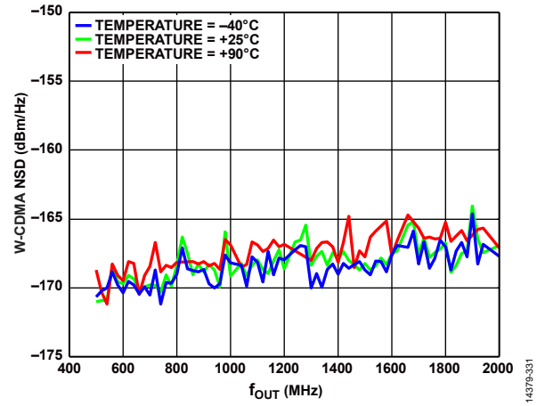
Figure 86. W-CDMA NSD Measured at 10% Offset from f_{OUT} vs. f_{OUT} over Temperature
