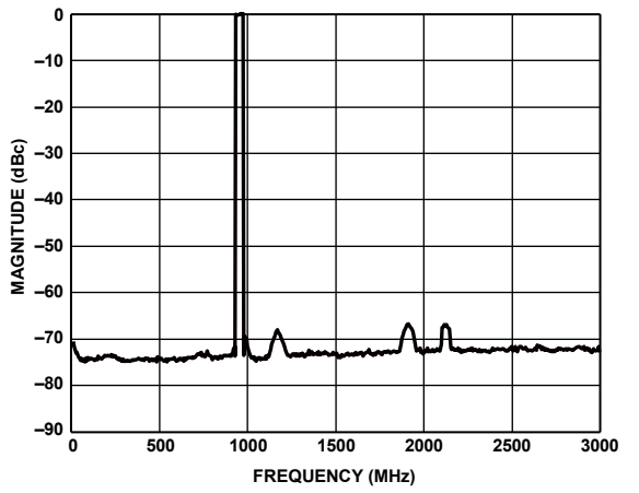
Figure 122. Eight Carriers at 950 MHz Output
