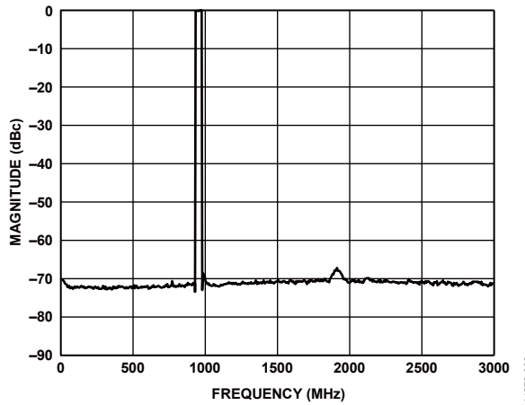
Figure 123. Eight Carriers at 950 MHz Output (Shuffle On)
