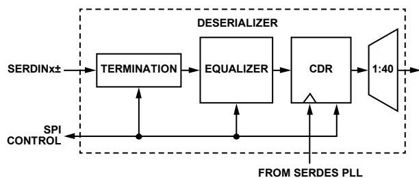
Figure 144. Deserializer Block Diagram
