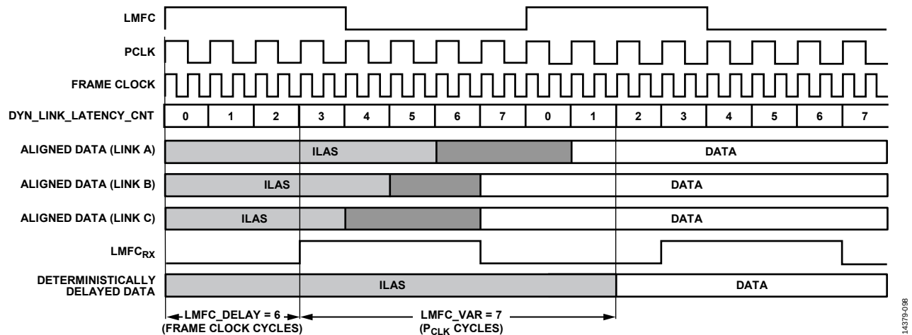
Figure 159. Multilink Synchronization Settings, Derived Method Example
