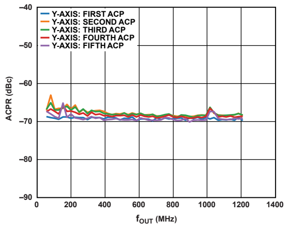
Figure 53. Eight-Carrier ACPR vs. f_{OUT}
