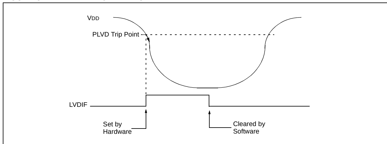
FIGURE 8-2: PLVD OPERATION
