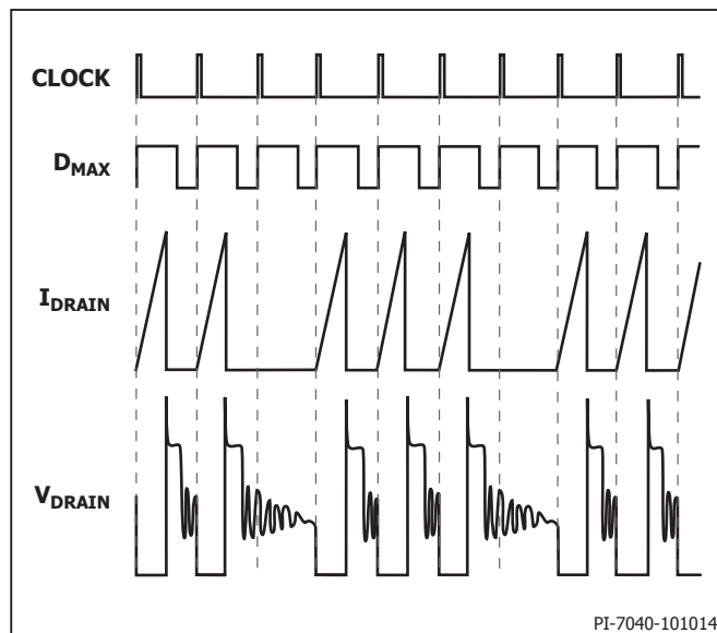
Figure 8. Operation at Moderately Heavy Loading.
