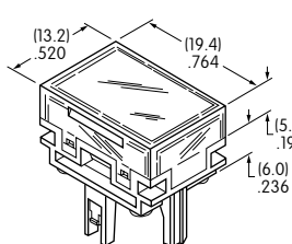
AT4163 Rectangular
