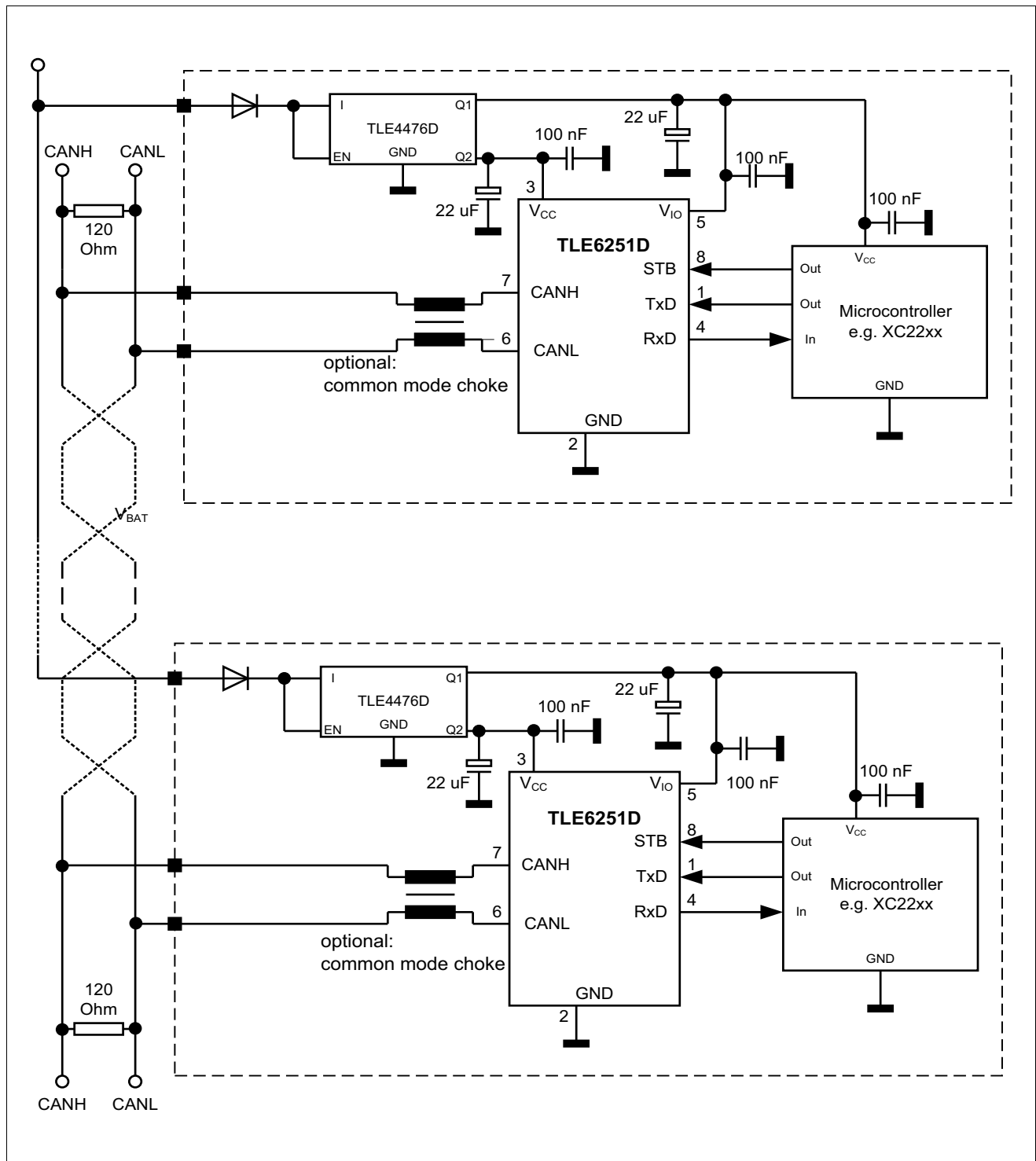
Figure 11 Application circuit
