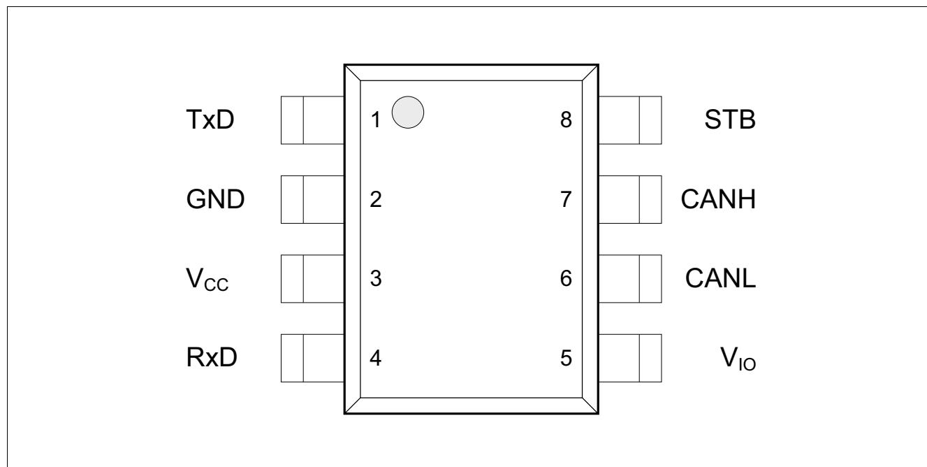
Figure 2 Pin configuration
