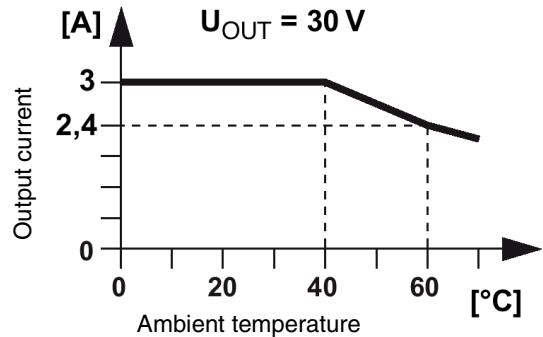
Figure 8 Temperature response
