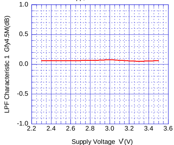
Low Pass Filter Characteristic 1 vs. Supply Voltage
