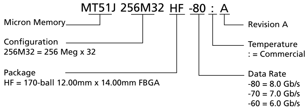
Figure 1: Part Numbering
