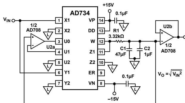
Figure 34. A Two-Chip, Wideband RMS-to-DC Converter
