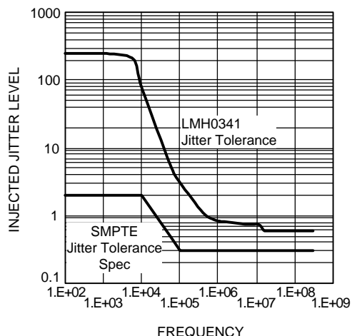
Figure 6. Jitter Tolerance Curve
