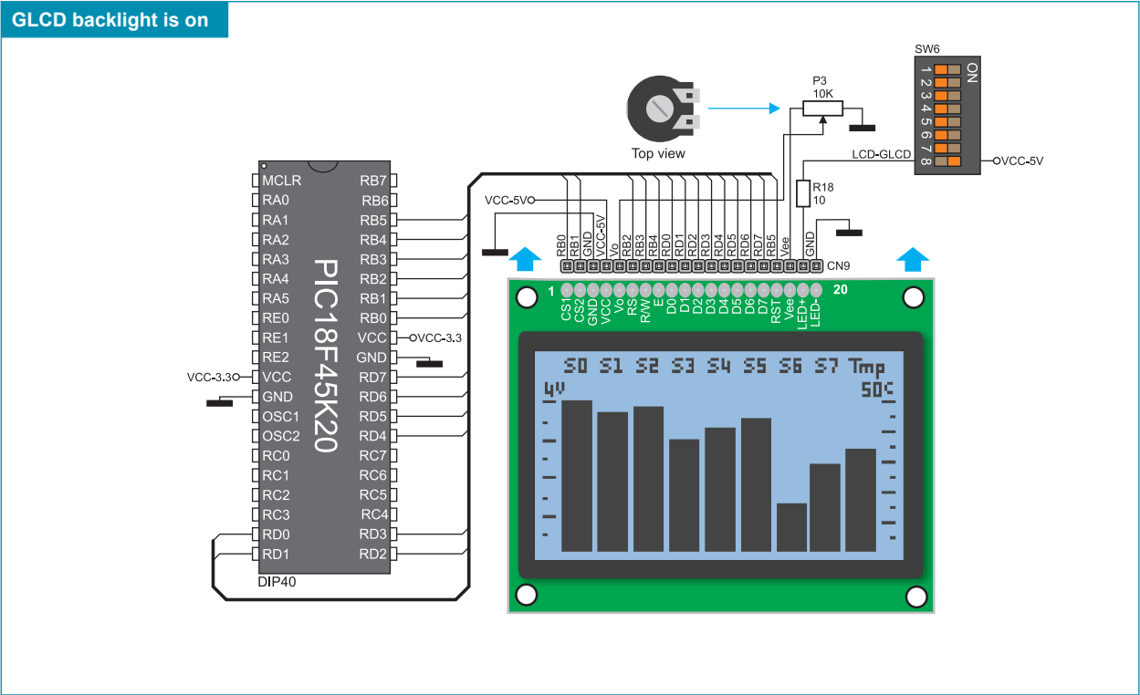
Figure 22-3: GLCD and microcontroller connection schematic
