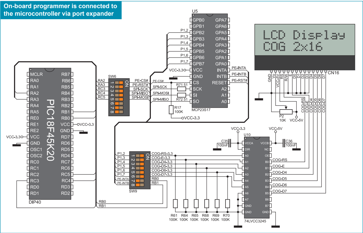
Figure 20-1: On-board 2x16 LCD
