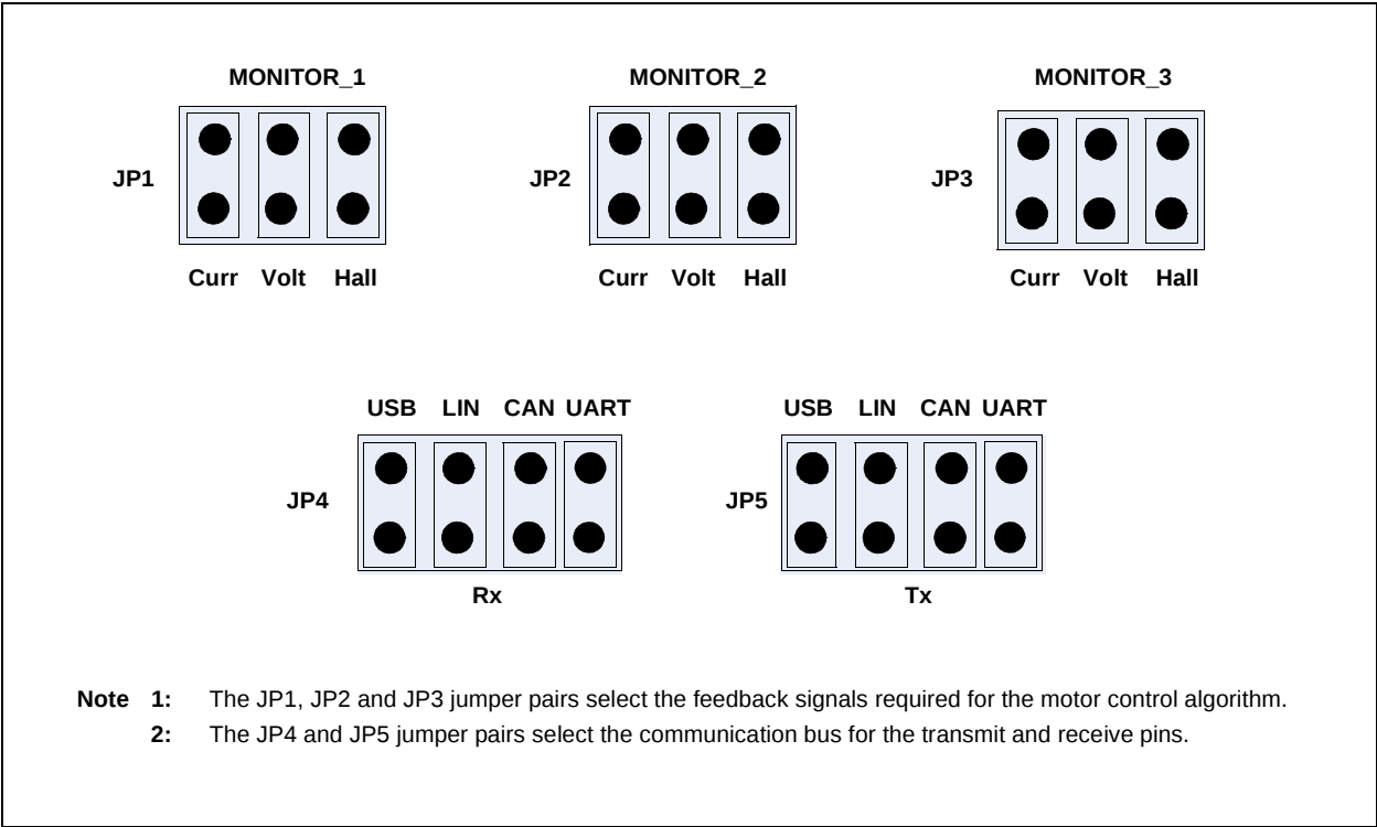
FIGURE 2-3: JUMPER SETTINGS
