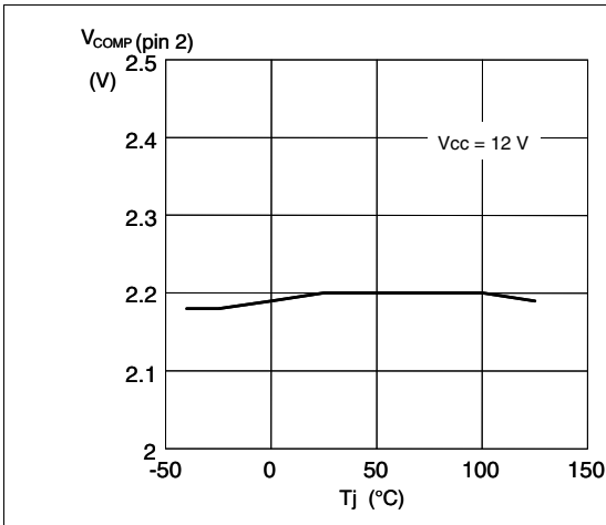
Figure 10. Static OVP level vs T_J
