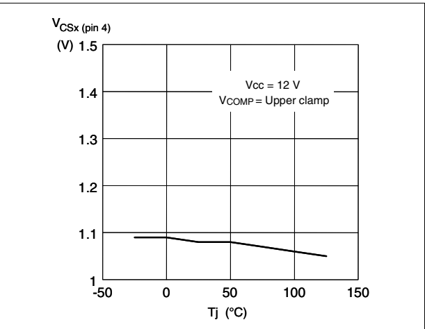
Figure 11. Vcs clamp vs T_J
