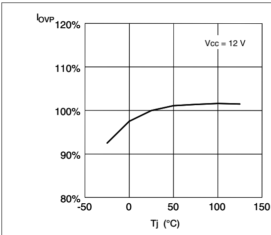
Figure 12. Dynamic OVP current vs T_J (normalized value)
