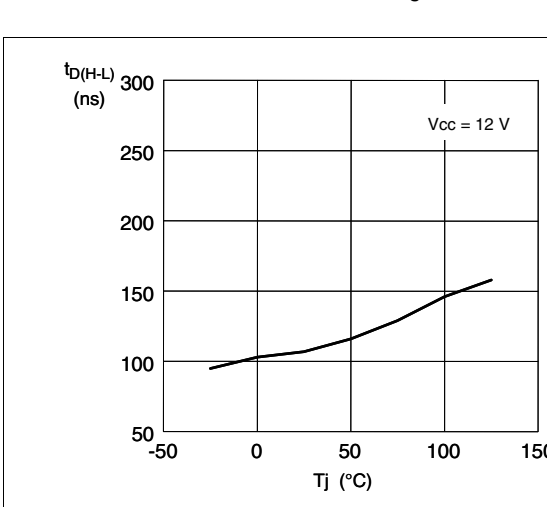
Figure 14. Delay-to-output vs T_J
