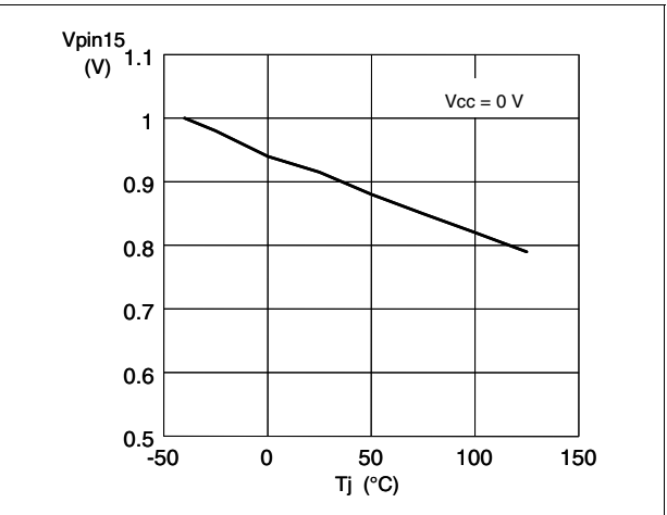
Figure 29. UVLO saturation vs T_J
