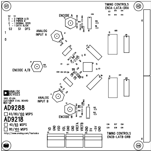
Figure 47. Top Silkscreen
