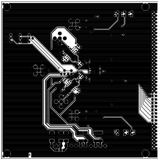
Figure 51. Bottom Routing
